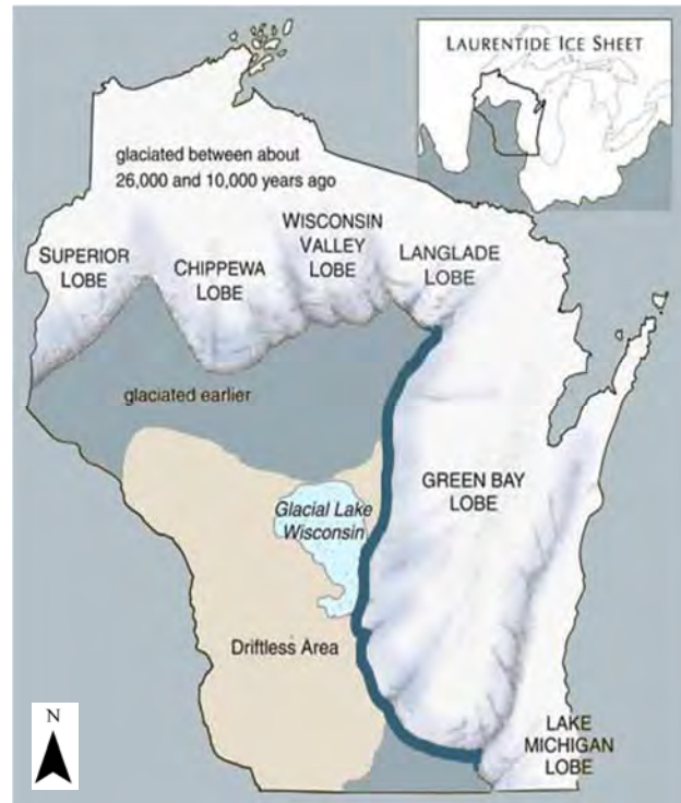
FIGURE 5 - ICE AGE GEOLOGY OF WISCONSIN.
